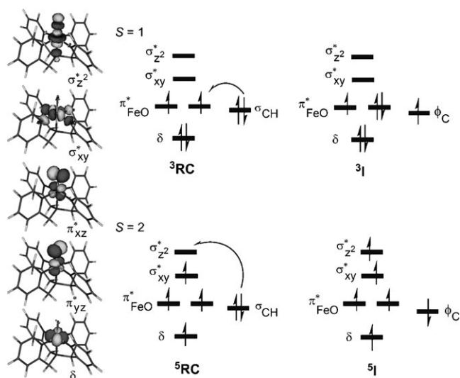
Figure 2. Orbital occupancy change during H-abstraction on the S=1 and S=2 states of an [\text{LFe}^{\text{IV}}\text{O}]^{2+} reagent (the drawn orbitals are specific to 2 ). The ^3/5\text{I} occupancies are related to the respective ^3/5\text{TS}_\text{H} .
